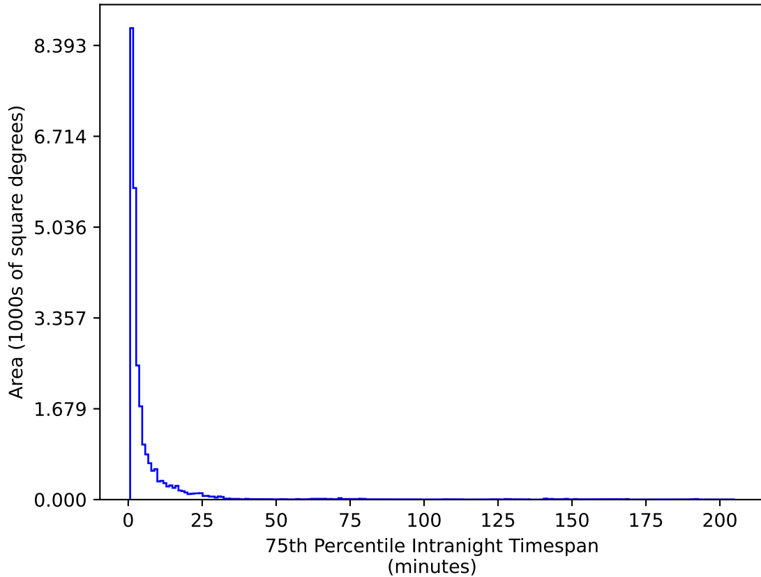
ddf_loaded_fl8_v3.4_10yrs All sky g band: 75th Percentile Intranight Timespan
