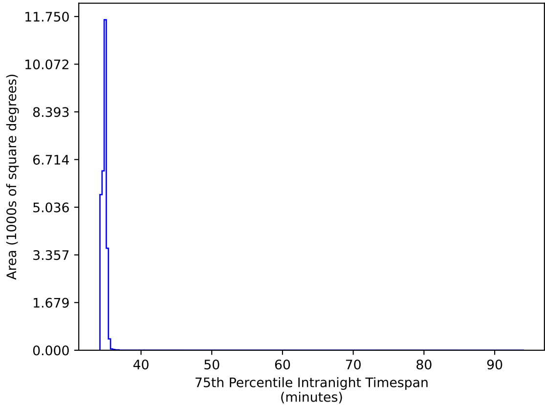
ddf_loaded_fl8_v3.4_10yrs All sky all bands: 75th Percentile Intranight Timespan
