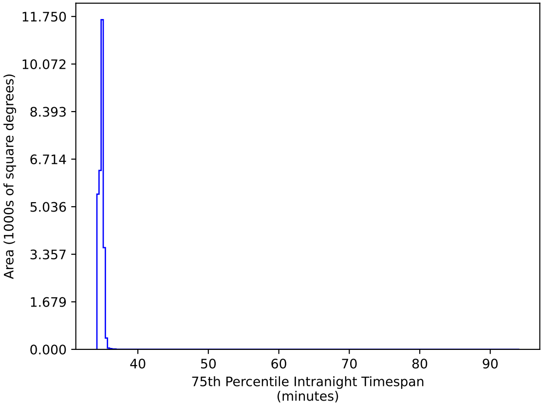
ddf_loaded_fl8_v3.4_10yrs All sky: 75th Percentile Intranight Timespan
