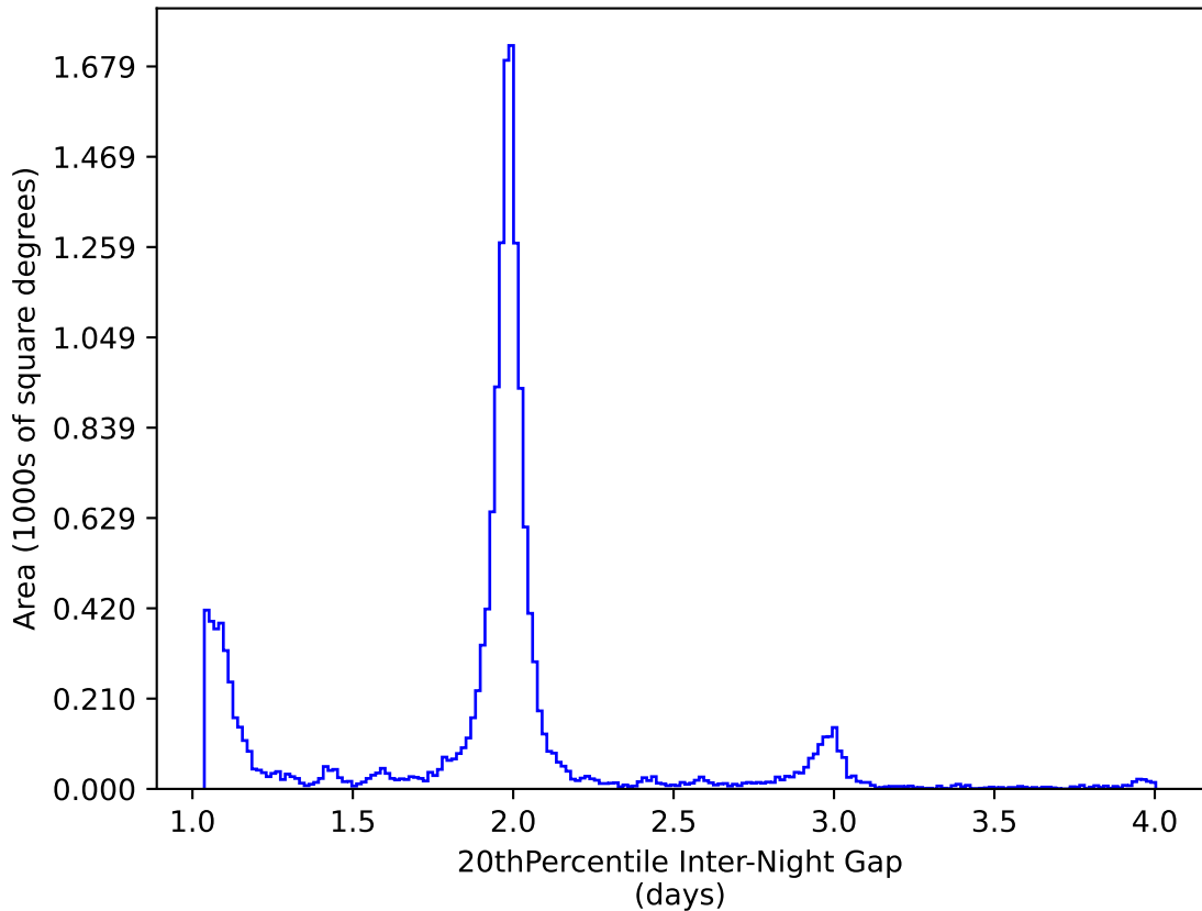
ddf_loaded_fl8_v3.4_10yrs WFD y band: 20thPercentile Inter-Night Gap
