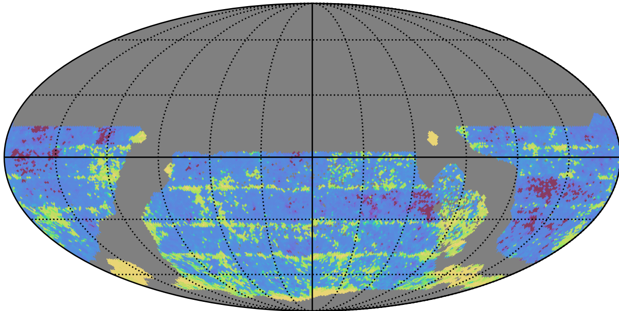
ddf_loaded_fl8_v3.4_10yrs WFD i band: 20thPercentile Inter-Night Gap
