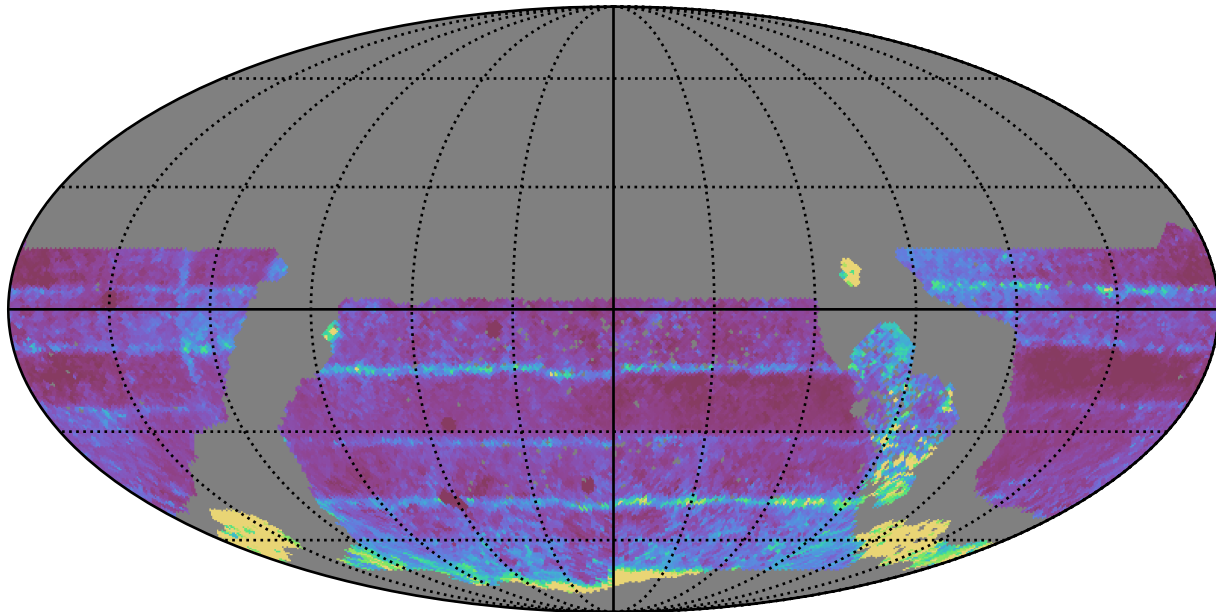
ddf_loaded_fl8_v3.4_10yrs WFD all bands: 20thPercentile Inter-Night Gap
