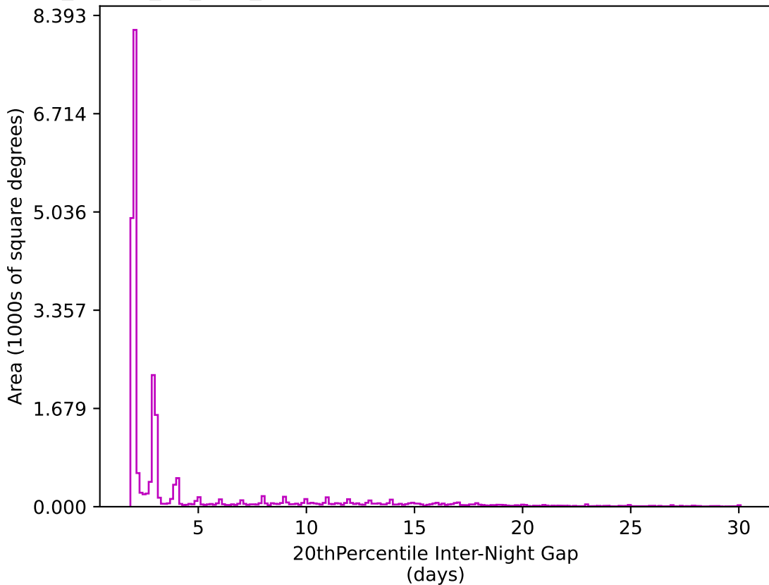
ddf_loaded_fl8_v3.4_10yrs All sky z band: 20thPercentile Inter-Night Gap
