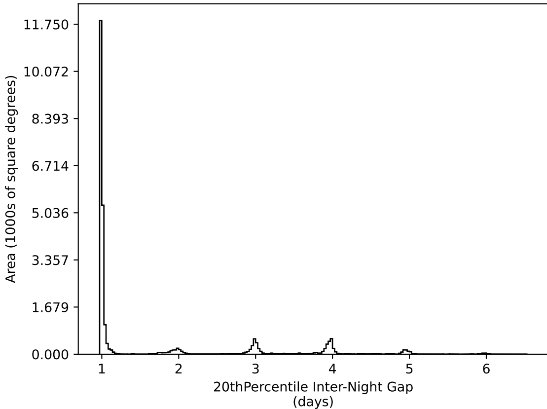
ddf_loaded_fl8_v3.4_10yrs All sky all bands: 20thPercentile Inter-Night Gap
