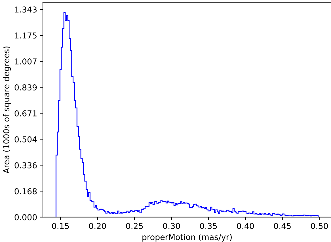
ddf_loaded_fl8_v3.4_10yrs : properMotion
