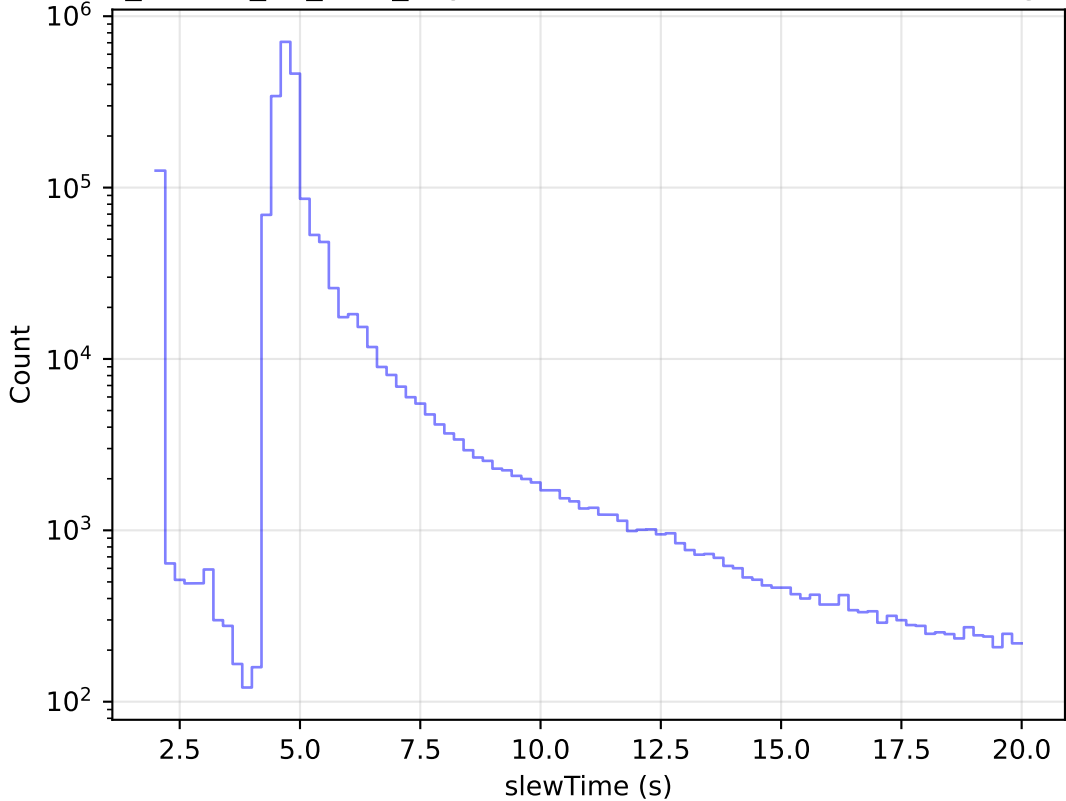
ddf_loaded_fl8_v3.4_10yrs All visits: Zoom Slew Time Histogram
