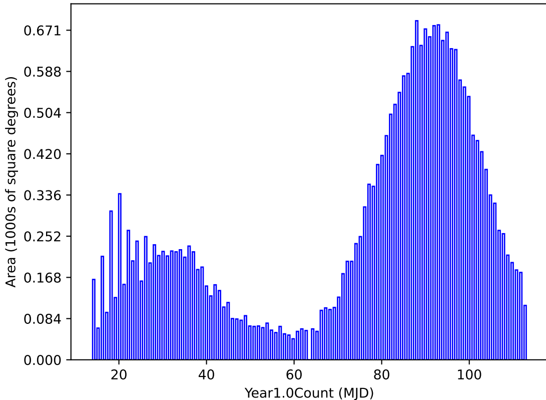
ddf_loaded_fl8_v3.4_10yrs night &lt; 365.25: Year1.0Count
