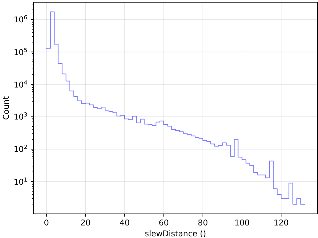
ddf_loaded_fl8_v3.4_10yrs All visits: Slew Distance Histogram
