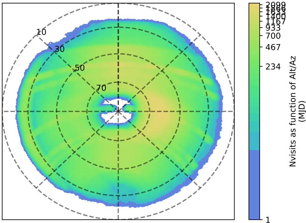
ddf_loaded_fl8_v3.4_10yrs r: Nvisits as function of Alt/Az
