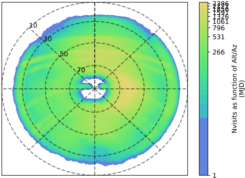
ddf_loaded_fl8_v3.4_10yrs i: Nvisits as function of Alt/Az
