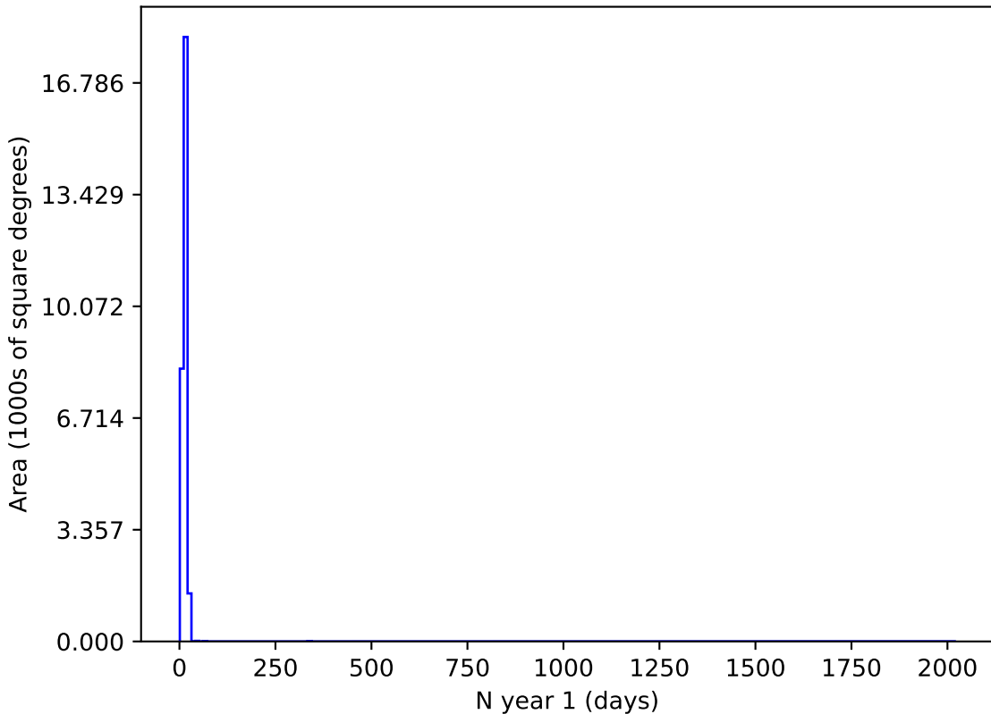
ddf_loaded_fl8_v3.4_10yrs z and night < 365: N year 1
