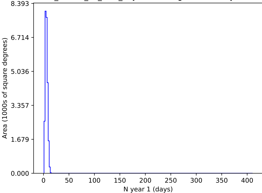
ddf_loaded_fl8_v3.4_10yrs u and night < 365: N year 1
