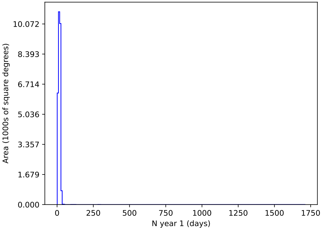
ddf_loaded_fl8_v3.4_10yrs r and night < 365: N year 1
