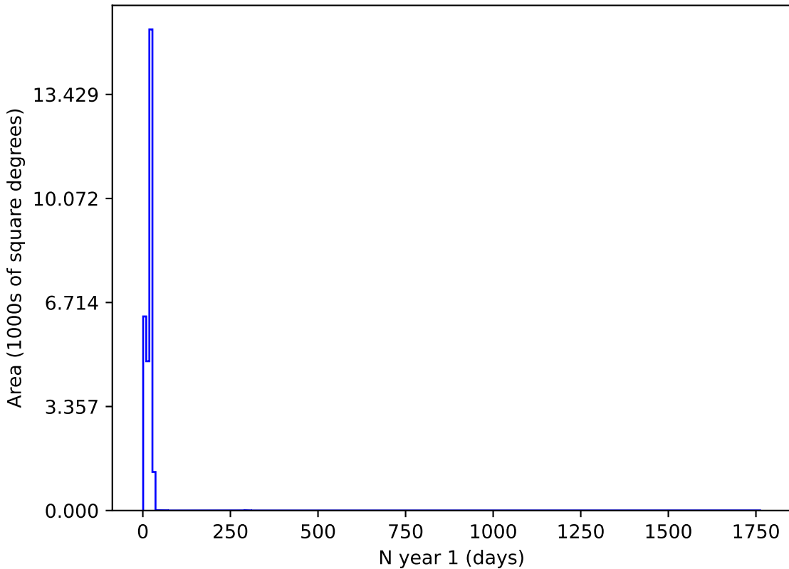
ddf_loaded_fl8_v3.4_10yrs i and night < 365: N year 1
