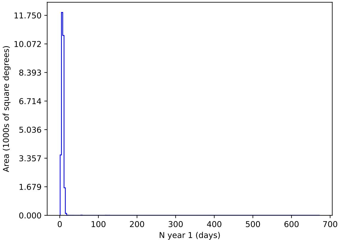
ddf_loaded_fl8_v3.4_10yrs g and night < 365: N year 1
