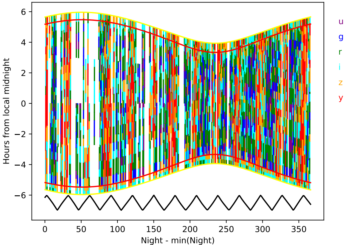
ddf_loaded_fl8_v3.4_10yrs year 9-10: Hourglass
