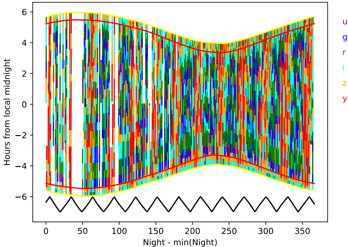
ddf_loaded_fl8_v3.4_10yrs year 6-7: Hourglass
