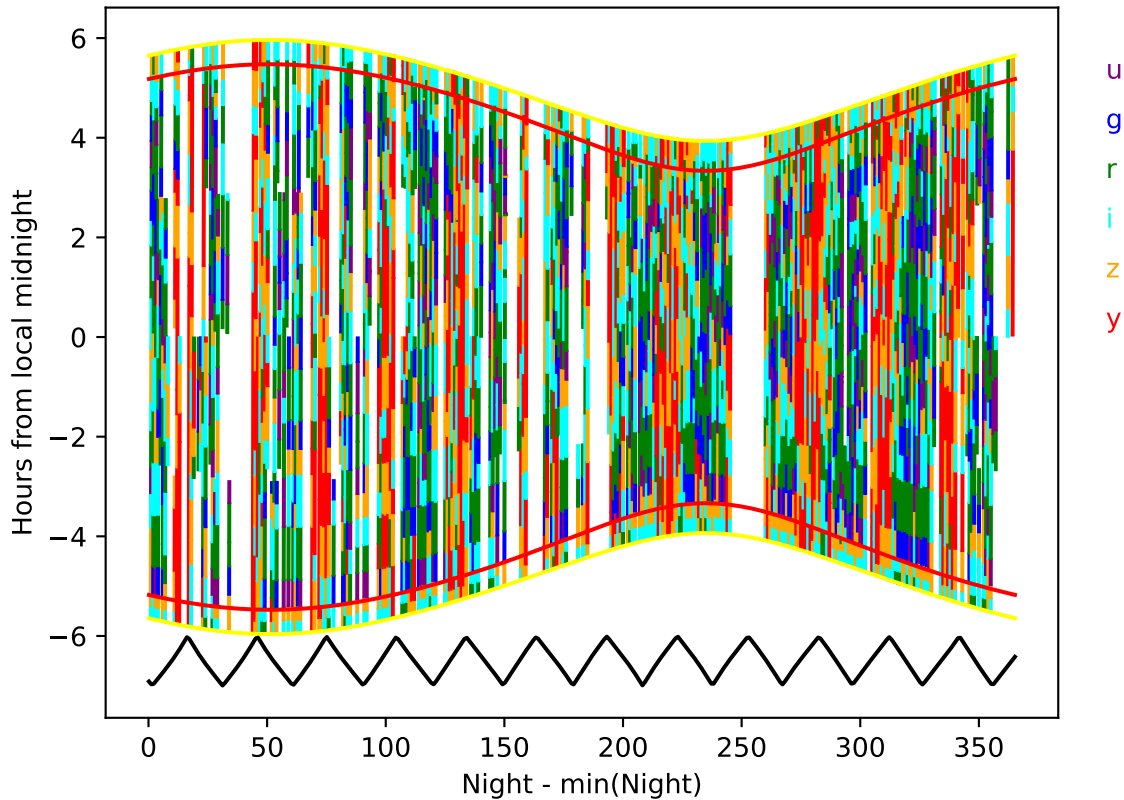
ddf_loaded_fl8_v3.4_10yrs year 5-6: Hourglass
