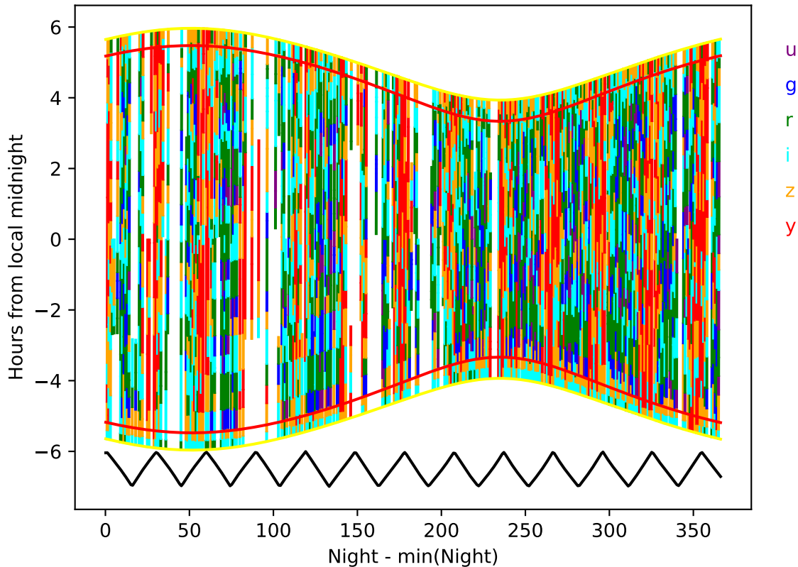
ddf_loaded_fl8_v3.4_10yrs year 1-2: Hourglass
