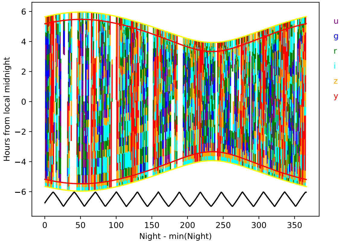
ddf_loaded_fl8_v3.4_10yrs year 0-1: Hourglass
