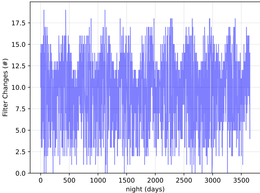
ddf_loaded_fl8_v3.4_10yrs : Filter Changes
