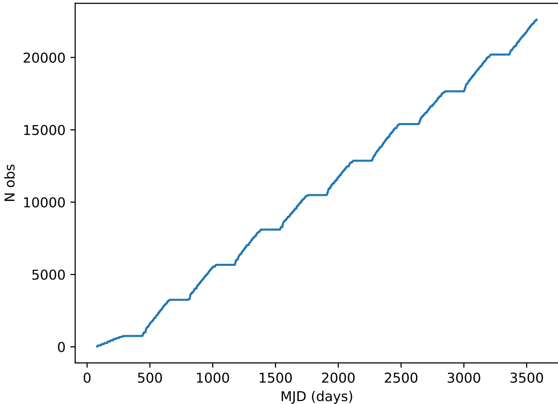
ddf_loaded_fl8_v3.4_10yrs note like DD:XMM_LSS%: Cumulative
