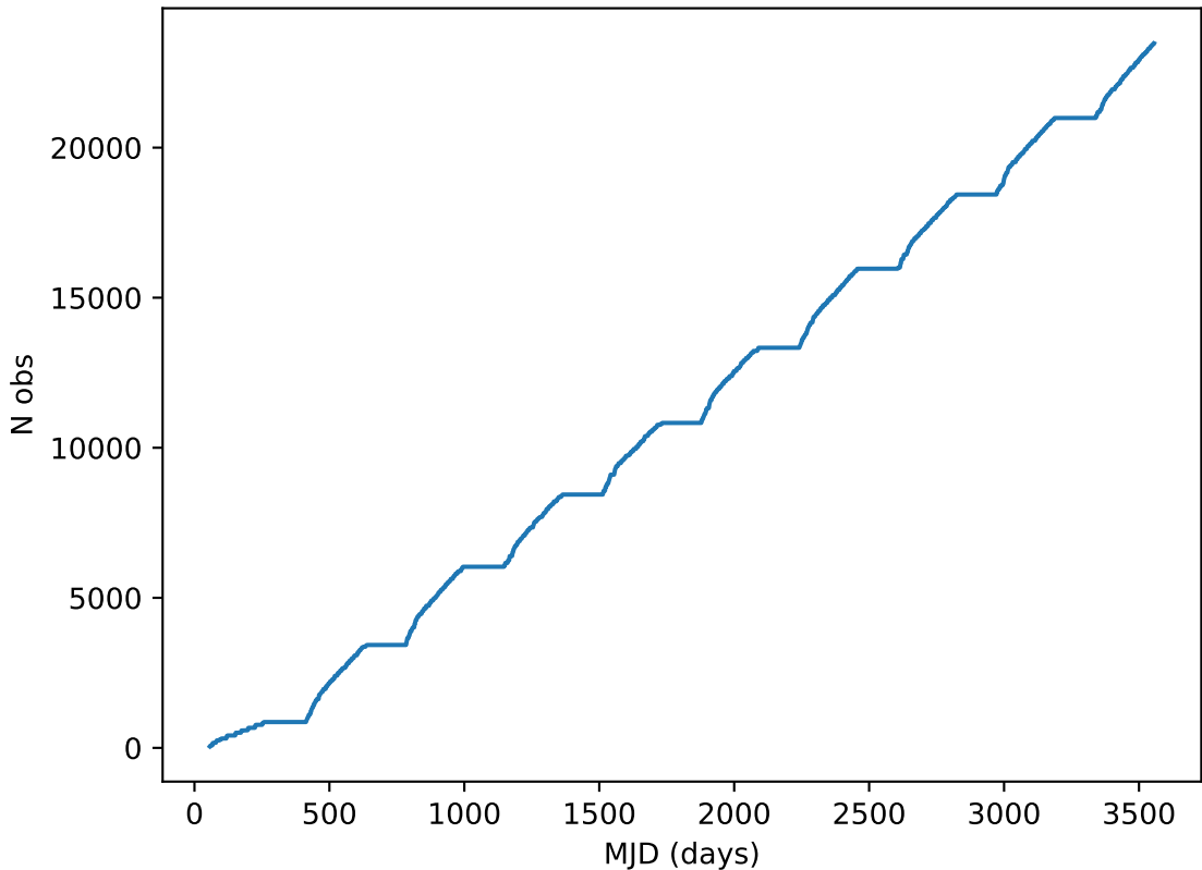
ddf_loaded_fl8_v3.4_10yrs note like DD:ELAISS1%: Cumulative
