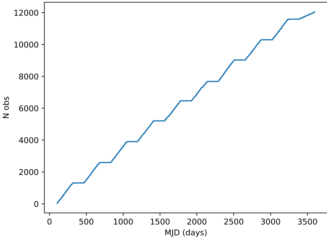
ddf_loaded_fl8_v3.4_10yrs note like DD:EDFS_a%: Cumulative
