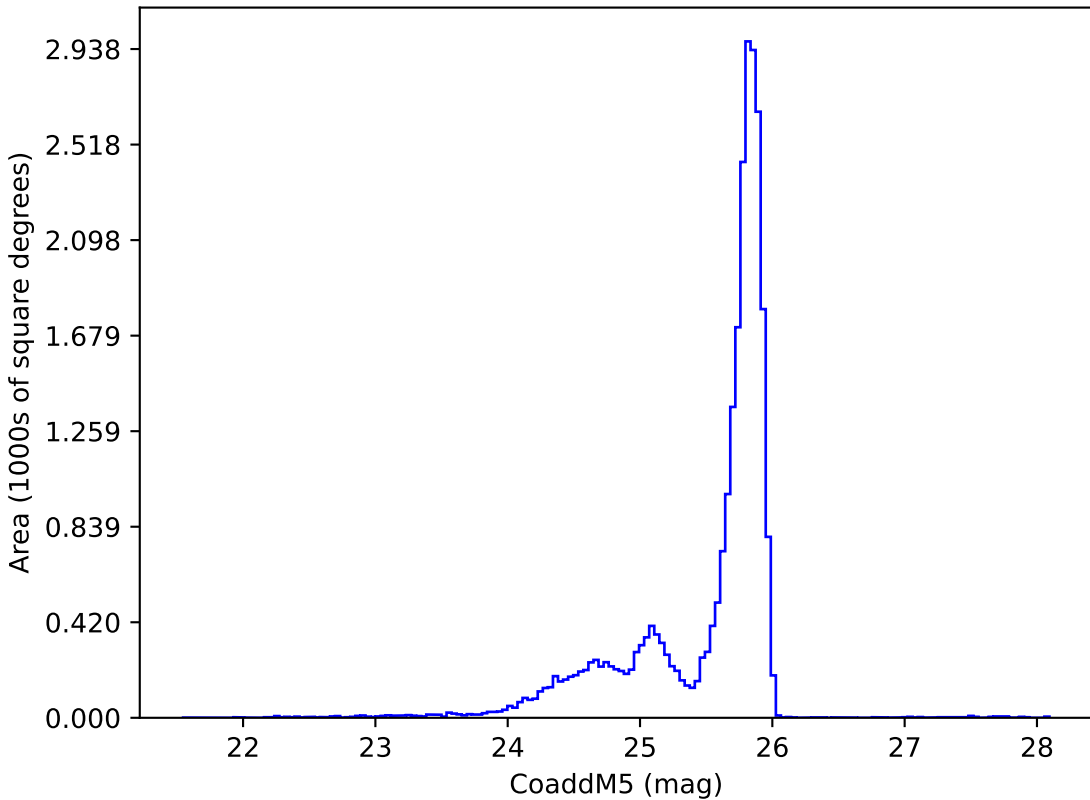
ddf_loaded_fl8_v3.4_10yrs z: CoaddM5
