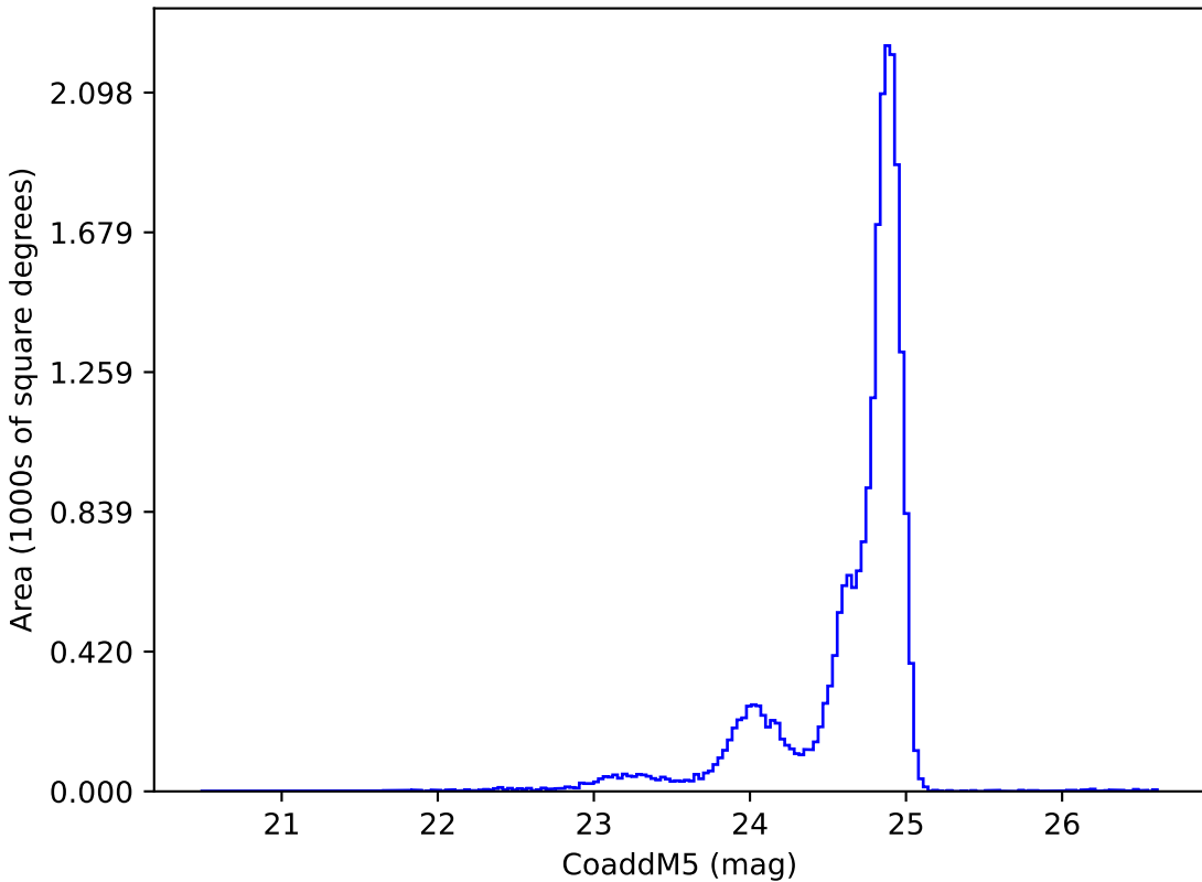
ddf_loaded_fl8_v3.4_10yrs y: CoaddM5
