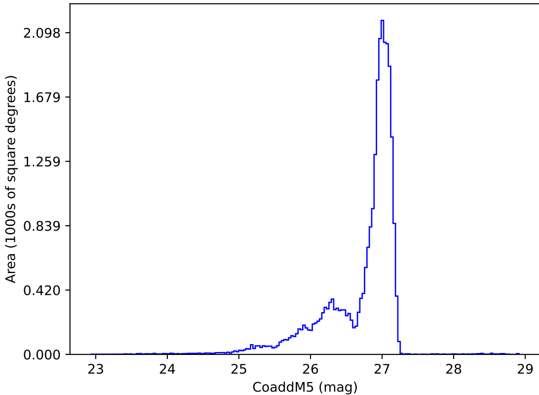
ddf_loaded_fl8_v3.4_10yrs r: CoaddM5
