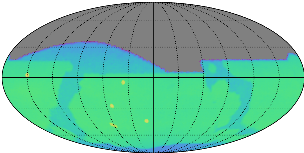
ddf_loaded_fl8_v3.4_10yrs i: CoaddM5
