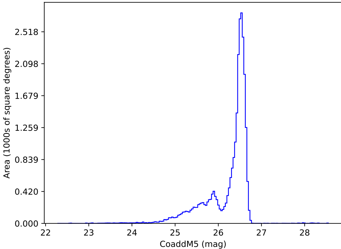
ddf_loaded_fl8_v3.4_10yrs i: CoaddM5
