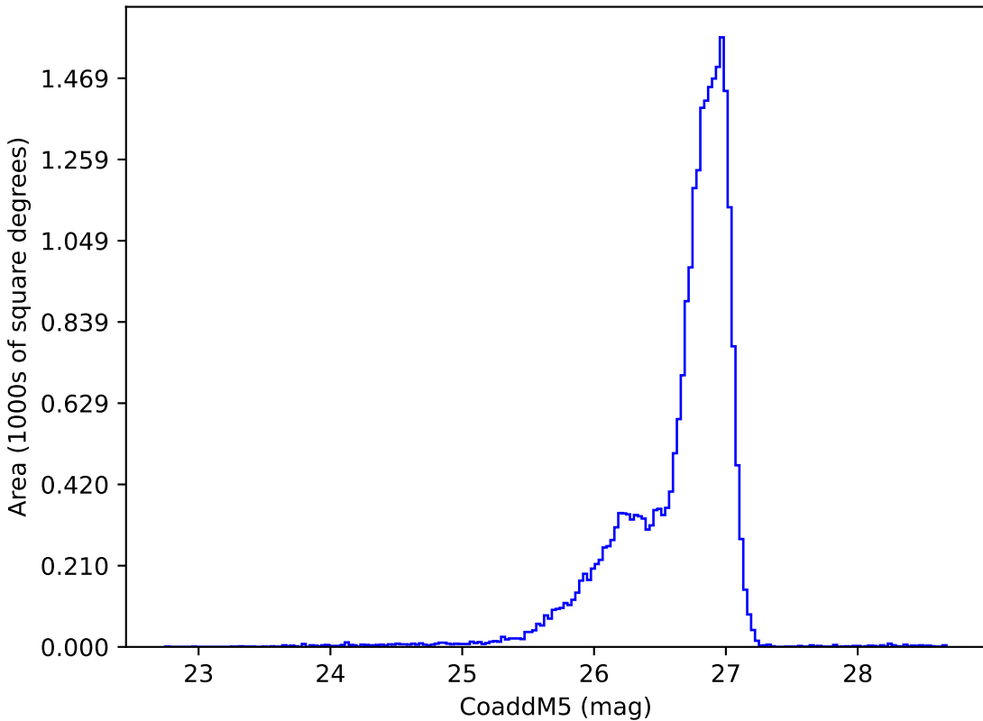
ddf_loaded_fl8_v3.4_10yrs g: CoaddM5
