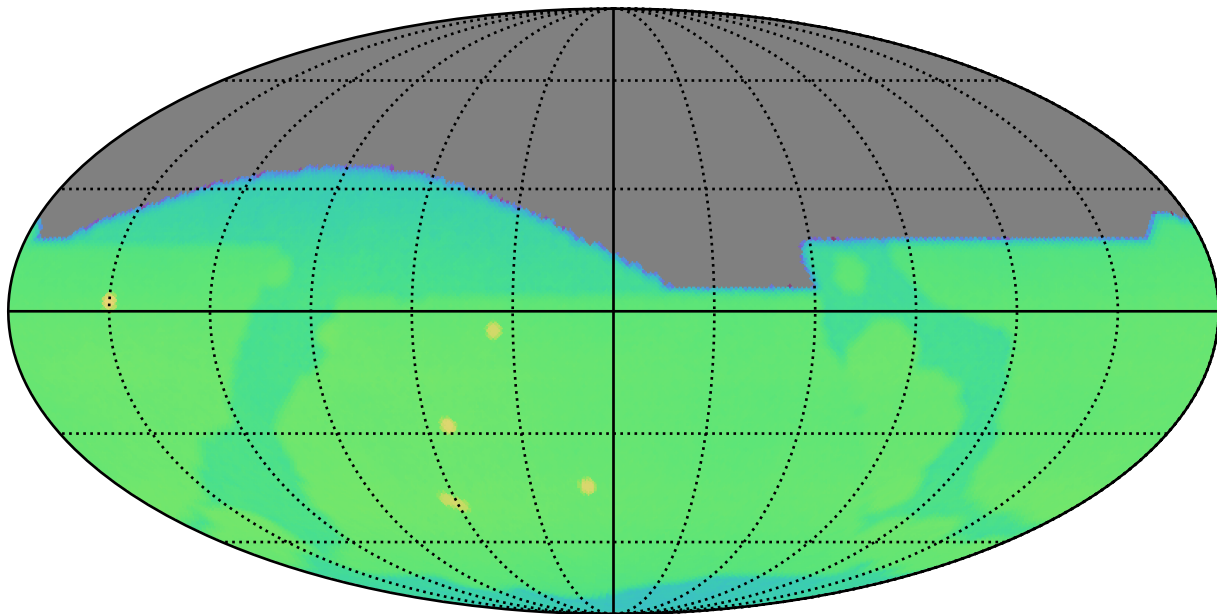
ddf_loaded_fl8_v3.4_10yrs : CoaddM5
