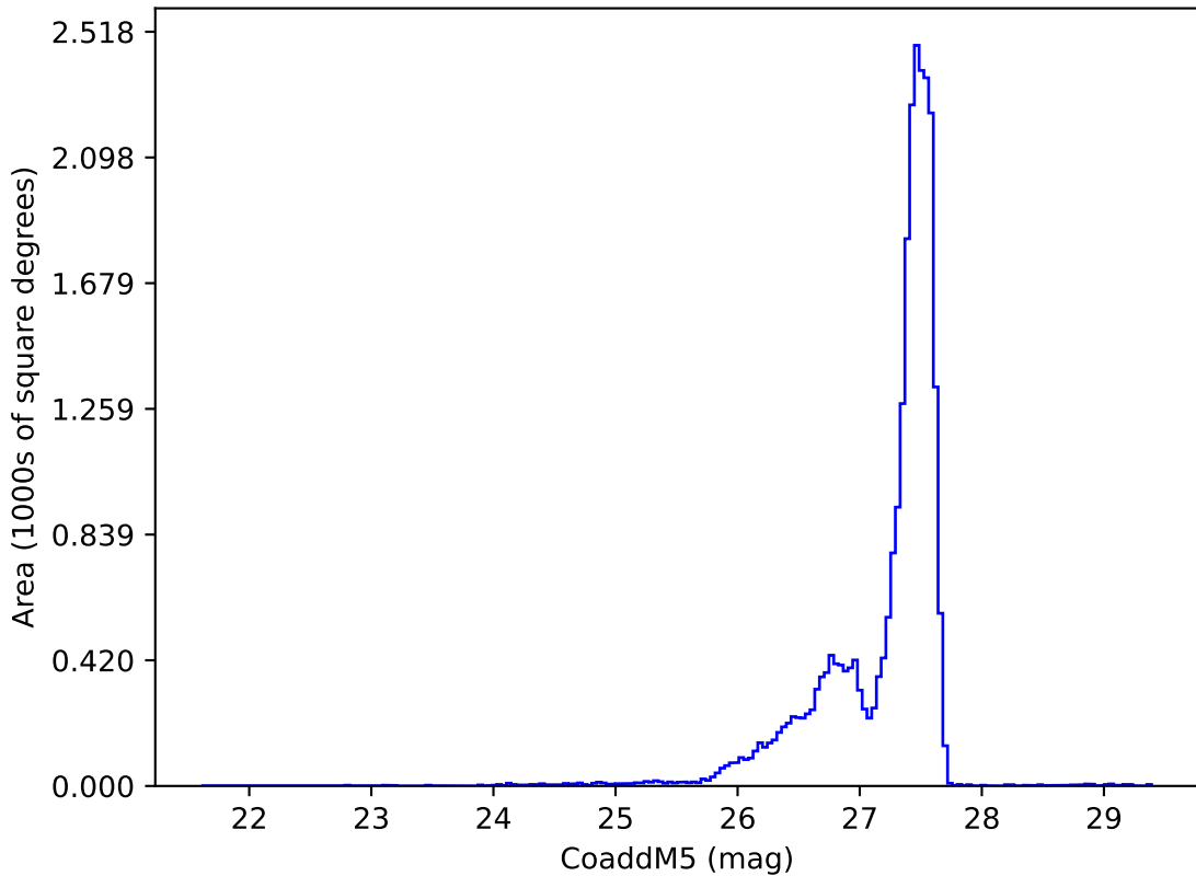
ddf_loaded_fl8_v3.4_10yrs : CoaddM5
