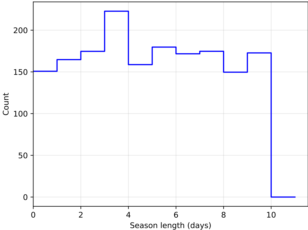
ddf_loaded_fl8_v3.4_10yrs DD:WFD all bands: SeasonLength
