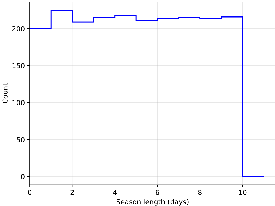
ddf_loaded_fl8_v3.4_10yrs DD:ELAISS1 all bands: SeasonLength
