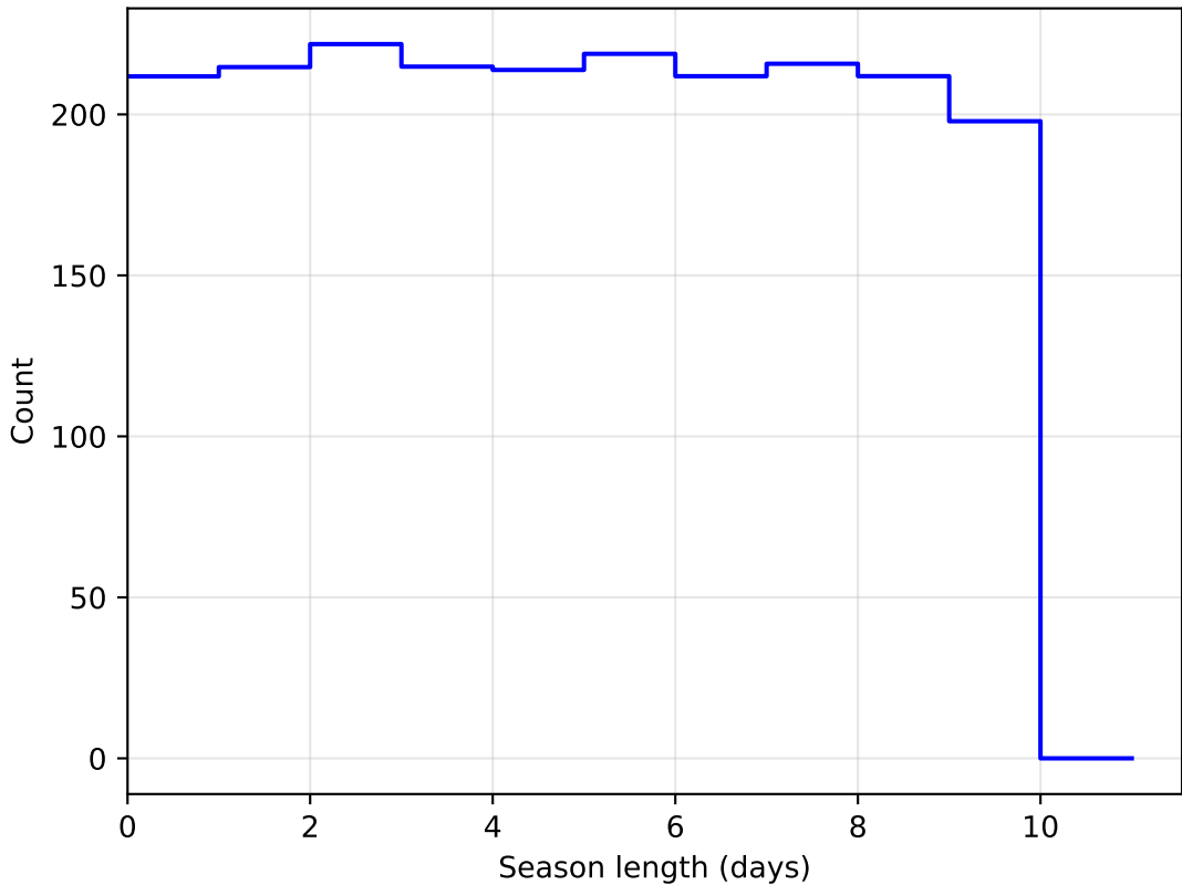
ddf_loaded_fl8_v3.4_10yrs DD:EDFS all bands: SeasonLength
