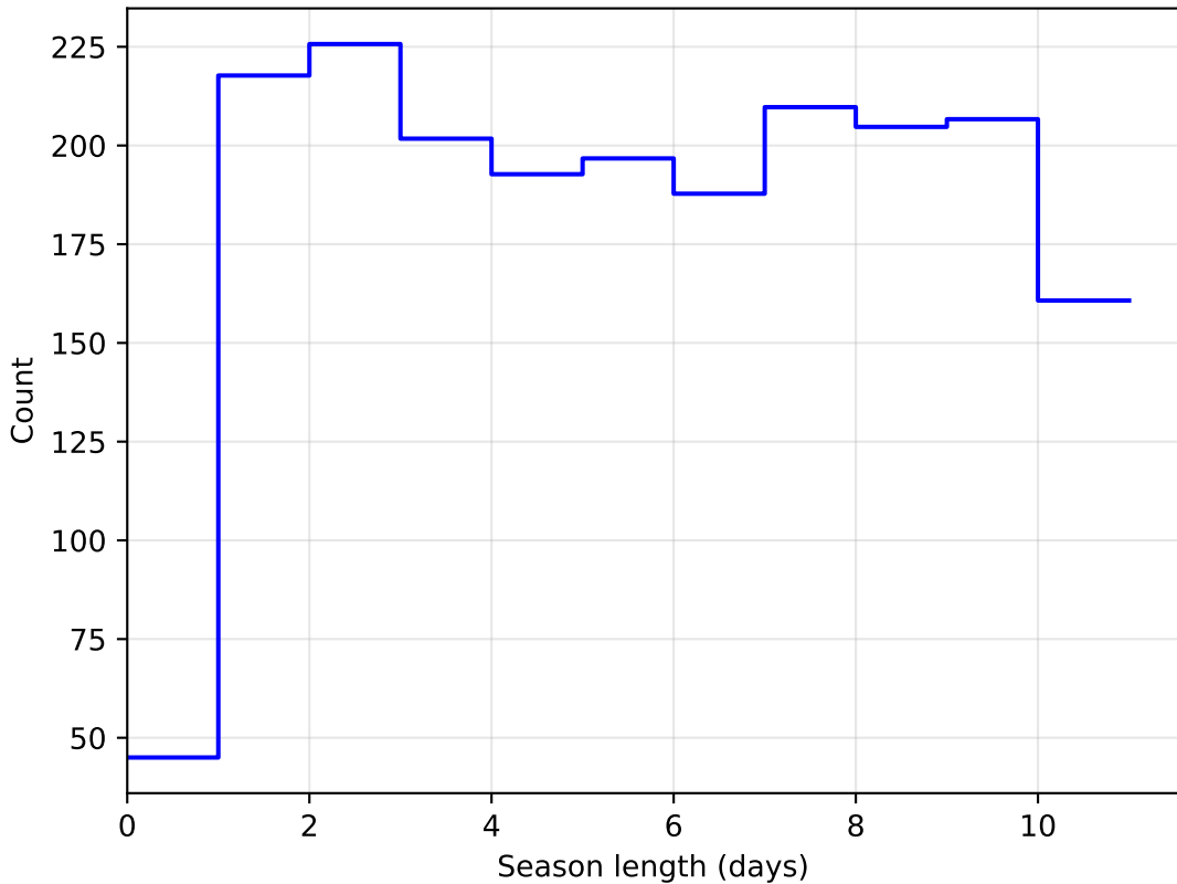
ddf_loaded_fl8_v3.4_10yrs DD: COSMOS all bands: SeasonLength
