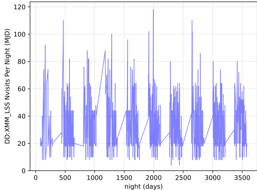
ddf_loaded_fl8_v3.4_10yrs all bands: DD:XMM_LSS Nvisits Per Night
