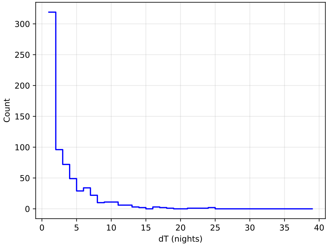
ddf_loaded_fl8_v3.4_10yrs all bands: DD:XMM_LSS Delta Nights Histogram
