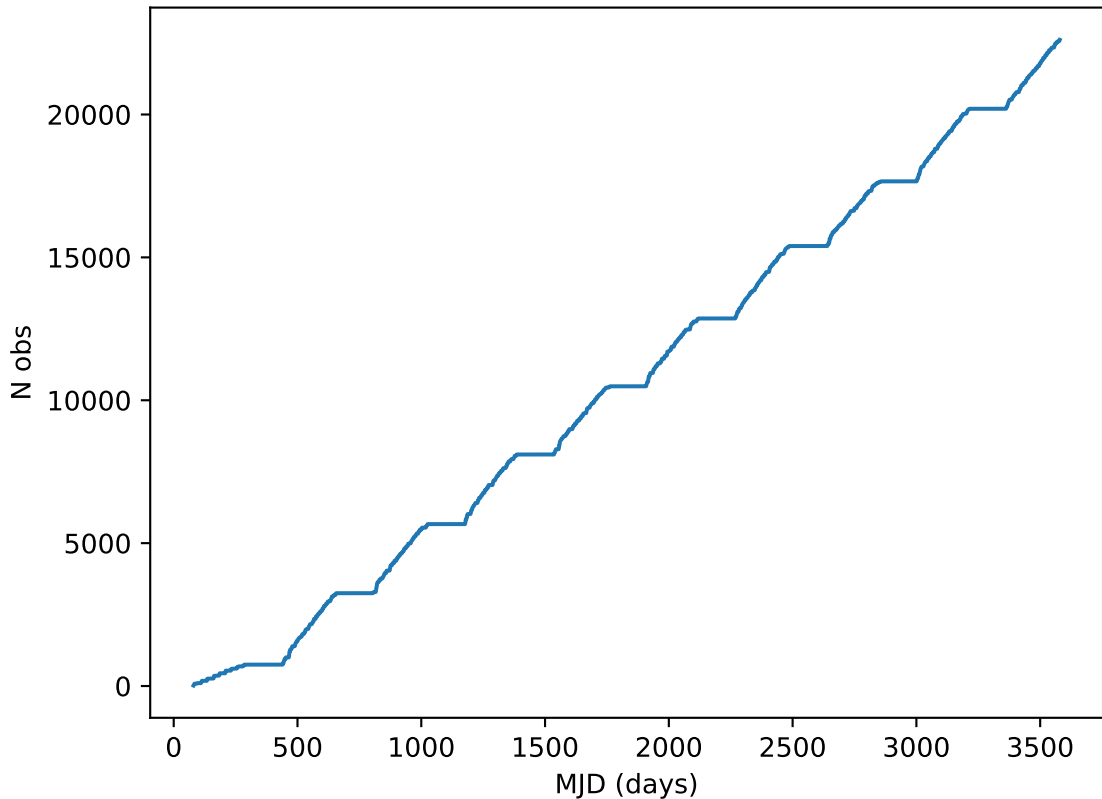
ddf_loaded_fl8_v3.4_10yrs all bands: DD:XMM_LSS Cumulative NVisits
