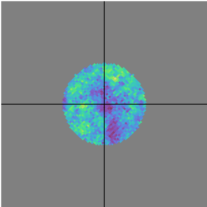
ddf_loaded_fl8_v3.4_10yrs u band: DD:WFD NVisits
