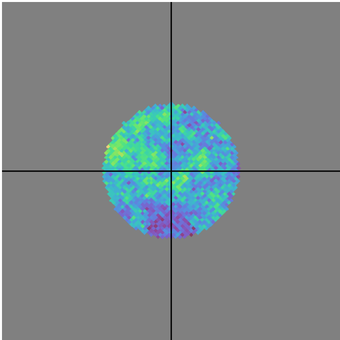
ddf_loaded_fl8_v3.4_10yrs g band: DD:WFD NVisits
