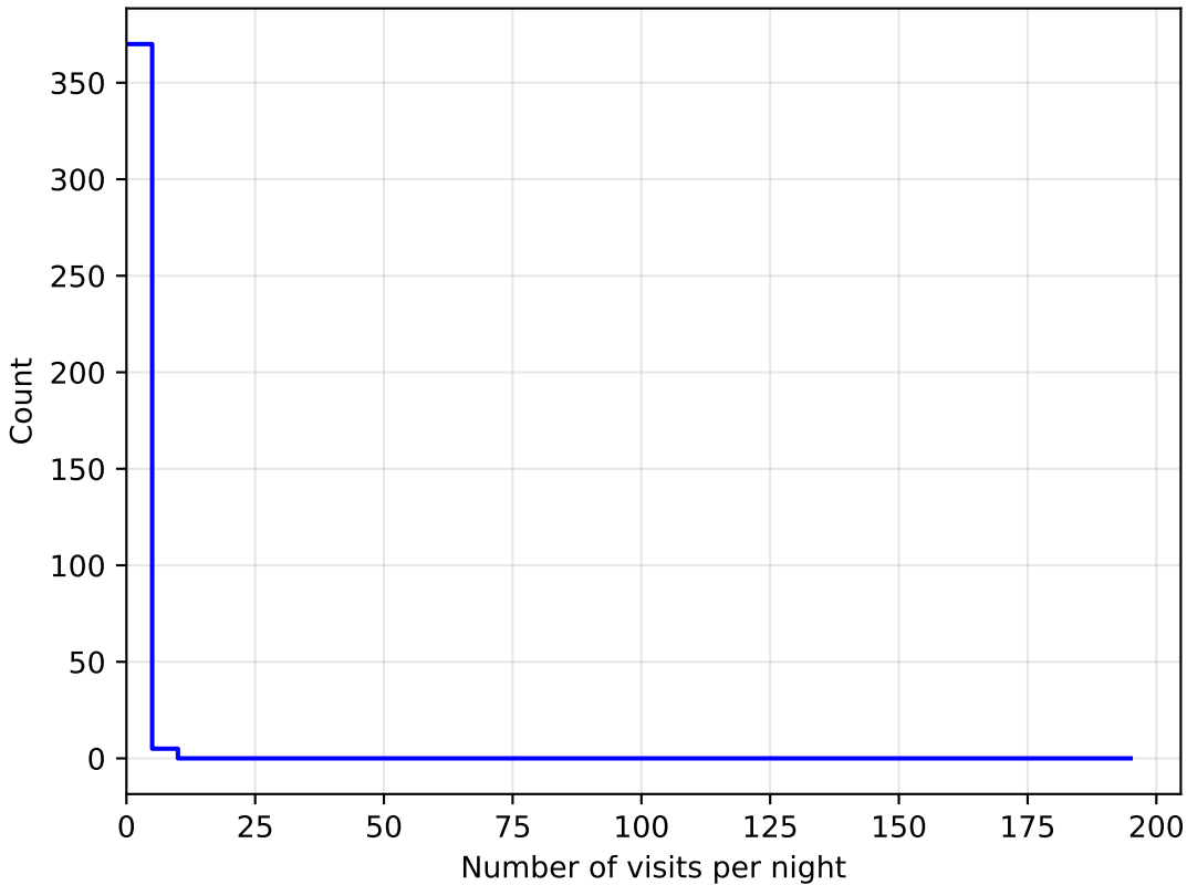
ddf_loaded_fl8_v3.4_10yrs all bands: DD:WFD NVisitsPerNight
