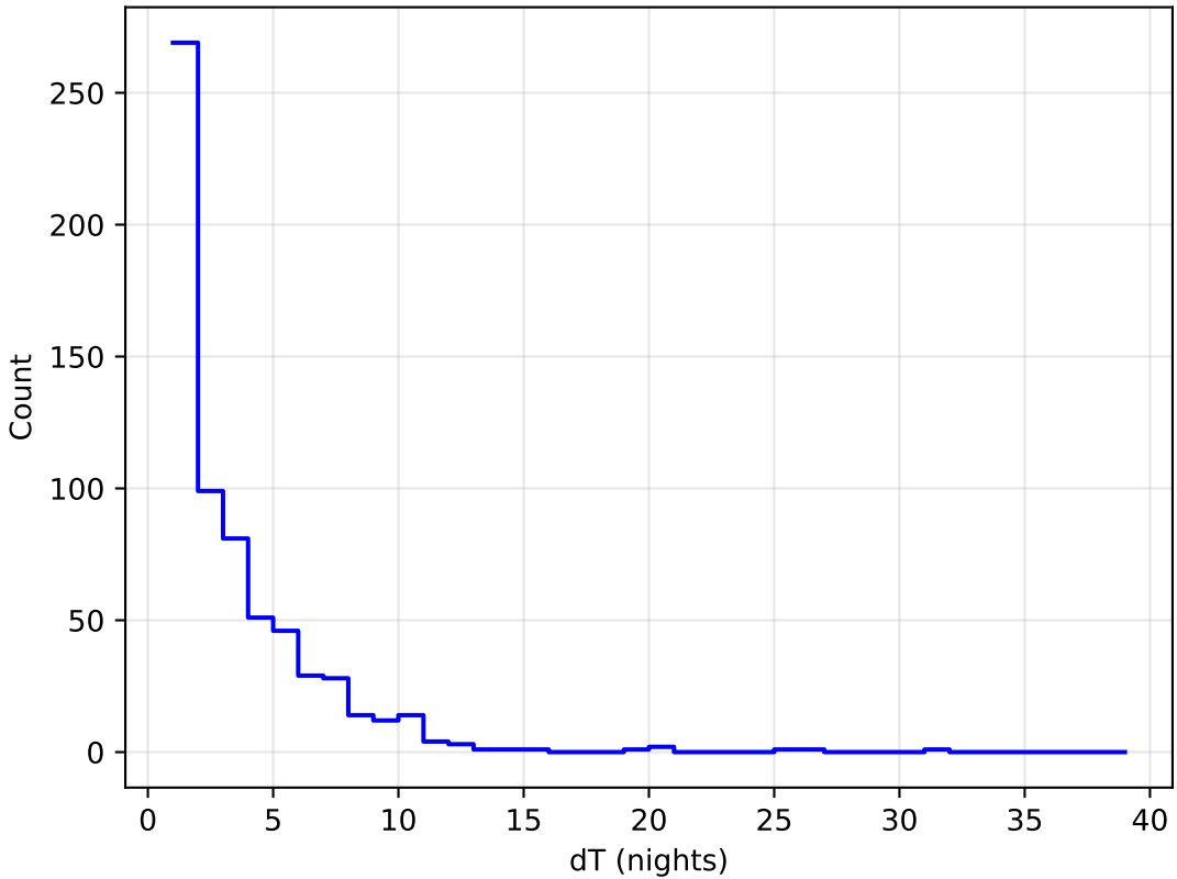
ddf_loaded_fl8_v3.4_10yrs all bands: DD:ELAISS1 Delta Nights Histogram
