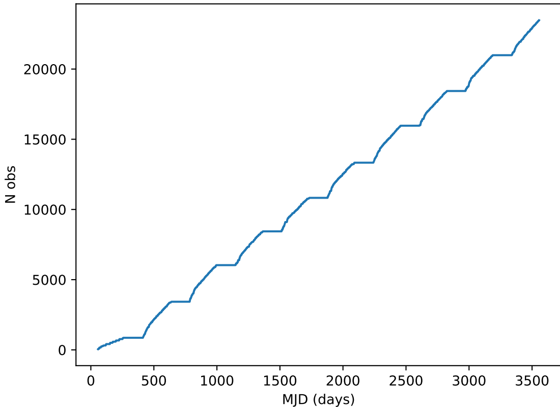
ddf_loaded_fl8_v3.4_10yrs all bands: DD:ELAISS1 Cumulative NVisits
