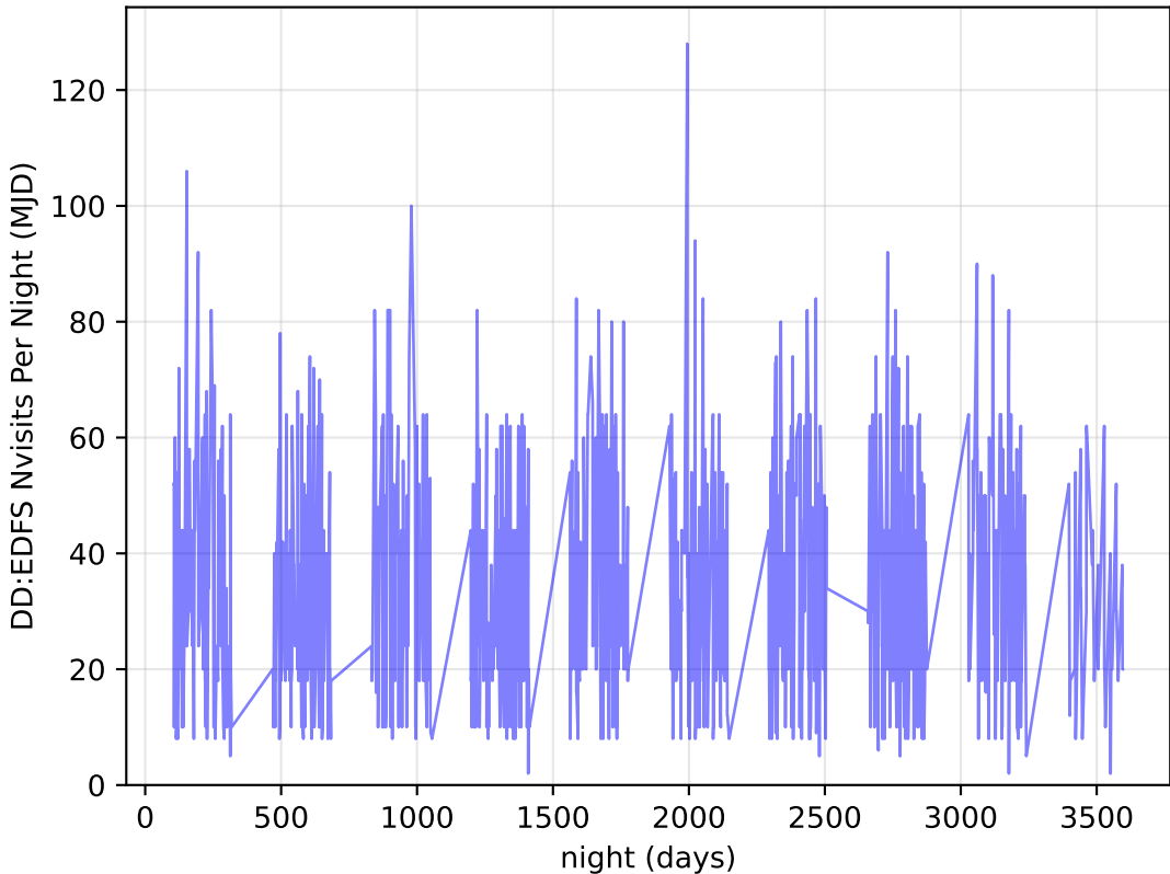
ddf_loaded_fl8_v3.4_10yrs all bands: DD:EDFS Nvisits Per Night
