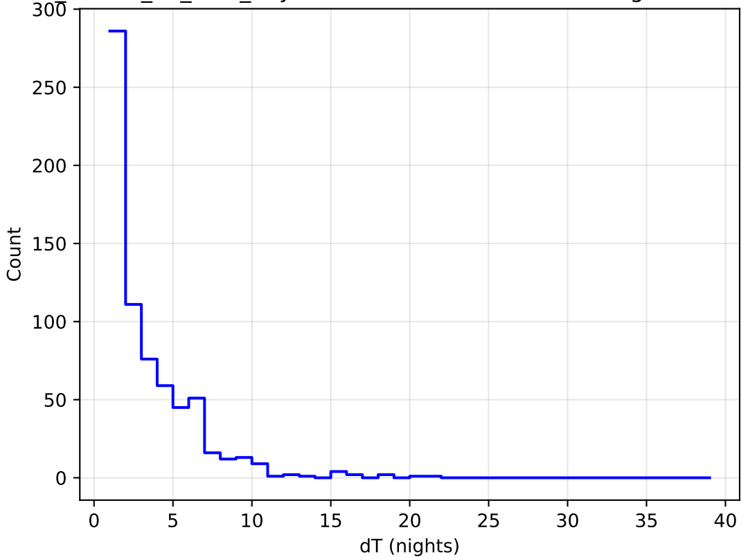
ddf_loaded_fl8_v3.4_10yrs all bands: DD:EDFS Delta Nights Histogram
